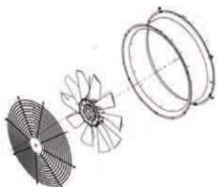
SINGLE PROPELLER
