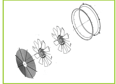
DOUBLE PROPELLER
